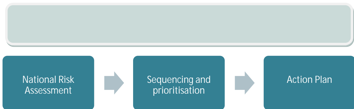
Figure 3. SIP framework
